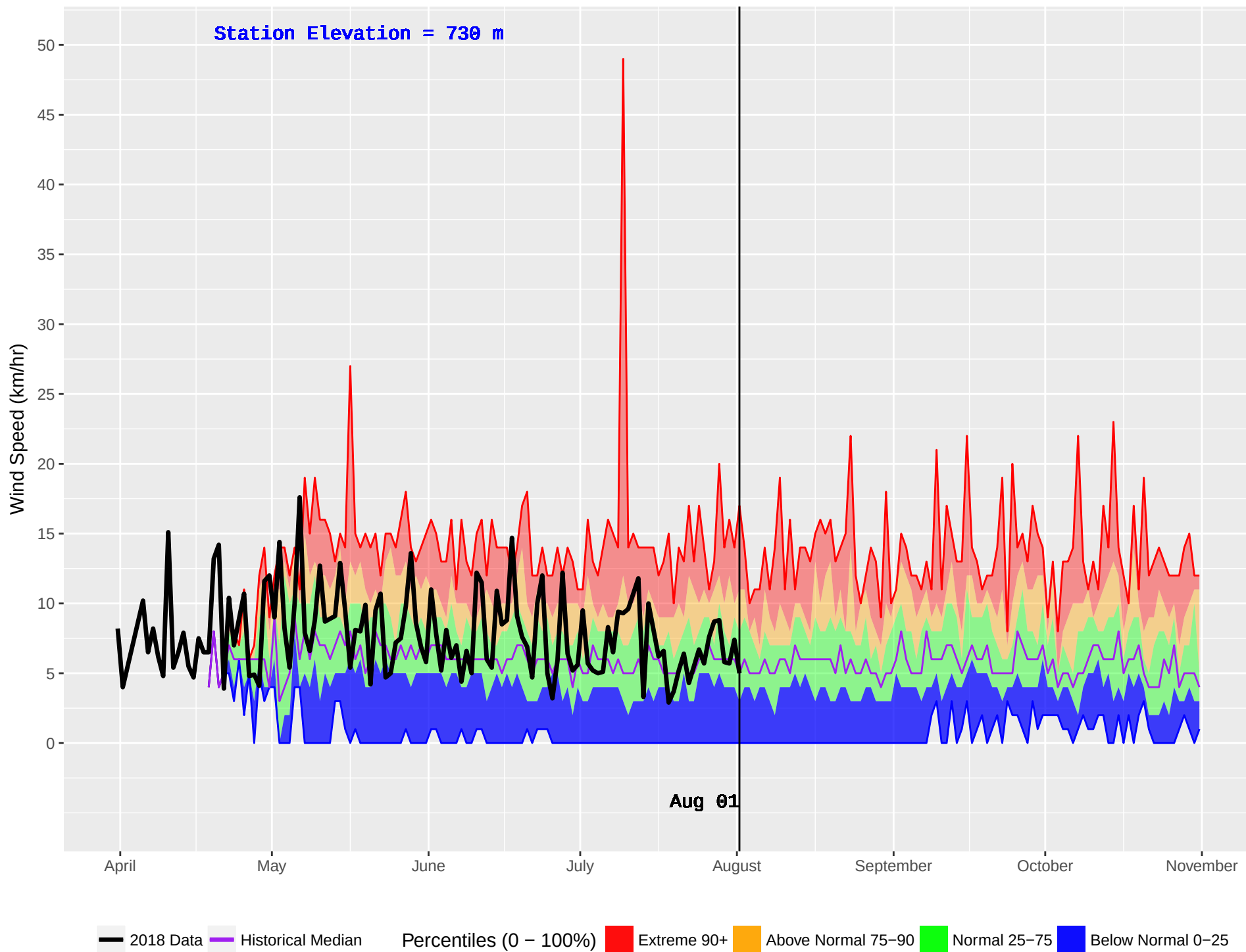
BOYA LAKE (445) : Historical (1985–2016) and Current (2018) Daily Wind Speed
