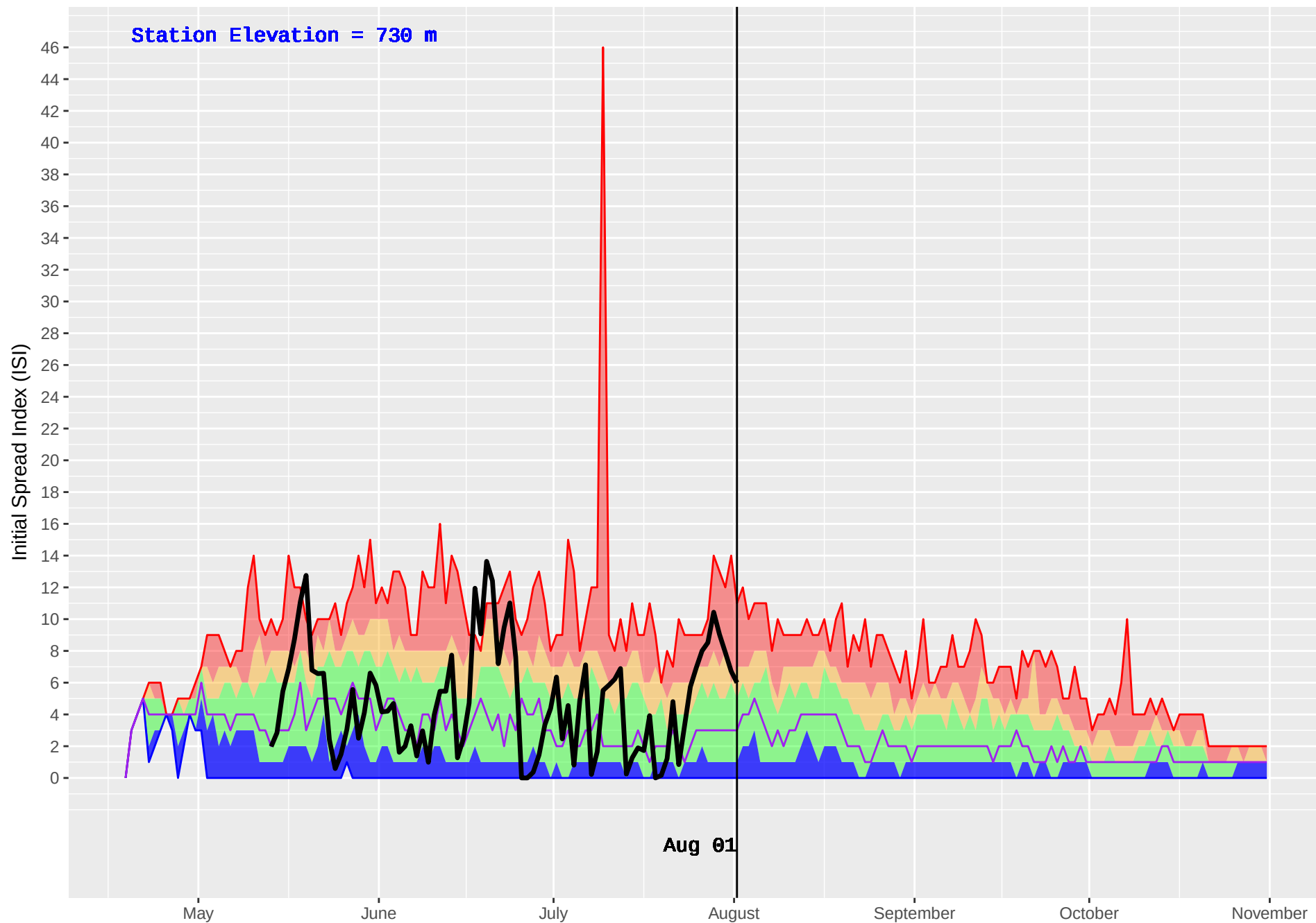
BOYA LAKE (445) : Historical (1985–2016) and Current (2018) Daily Initial Spread Index (ISI)
