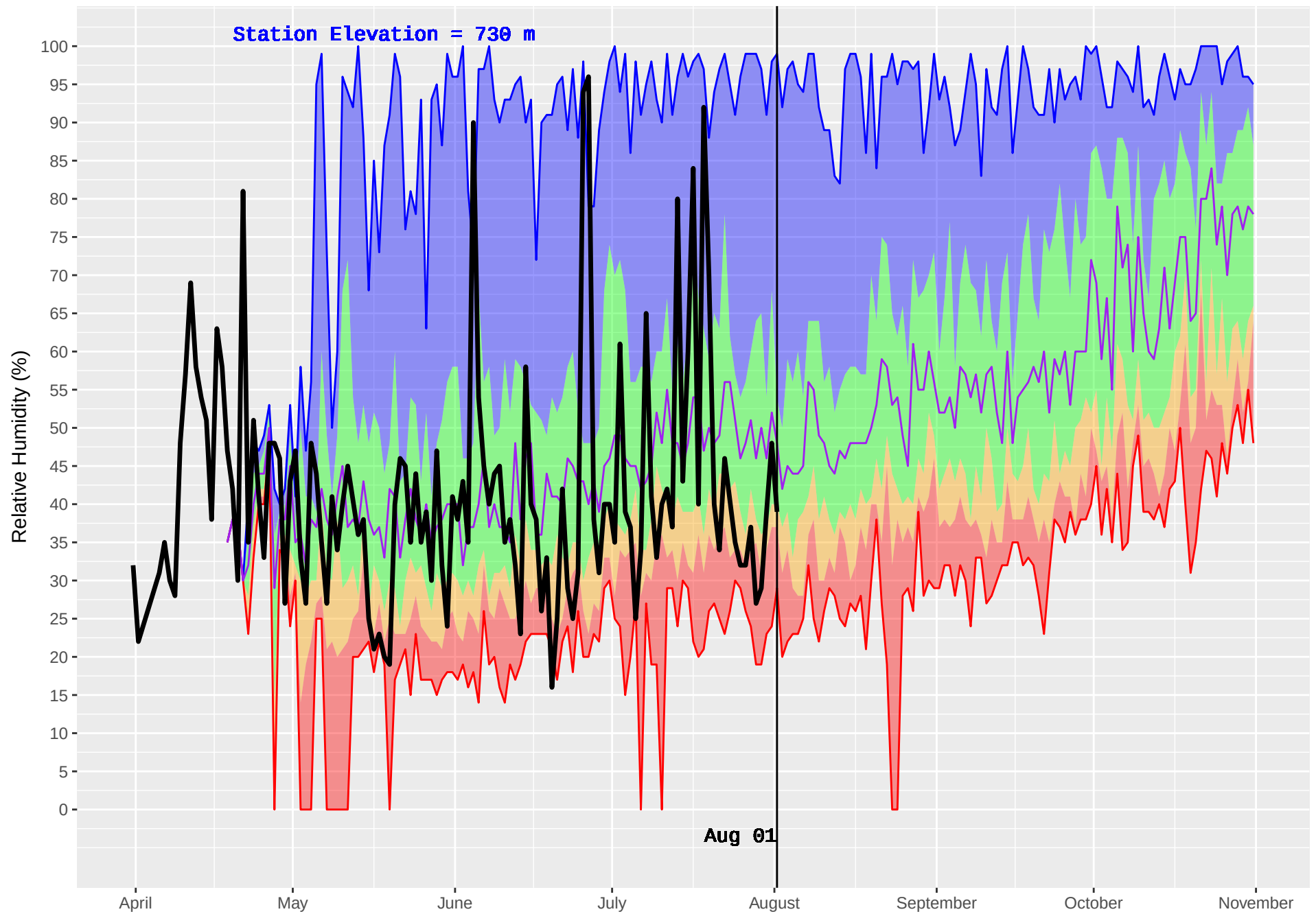
BOYA LAKE (445) : Historical (1985–2016) and Current (2018) Daily Relative Humidity
