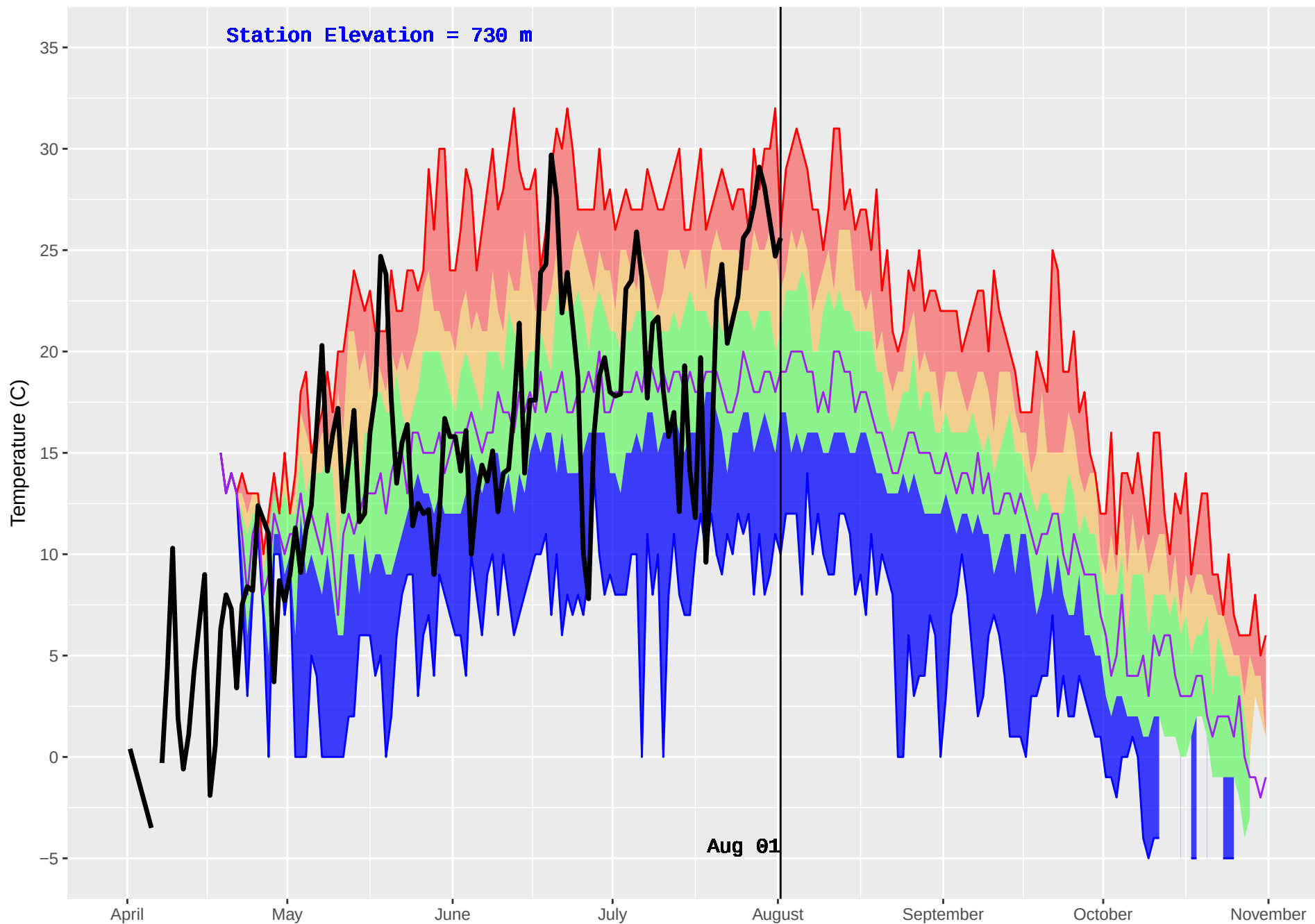
BOYA LAKE (445) : Historical (1985–2016) and Current (2018) Daily Temperature
