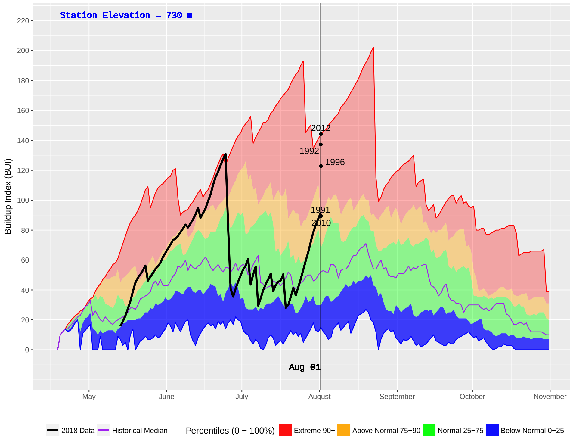
BOYA LAKE (445) : Historical (1985–2016) and Current (2018) Daily Buildup Index (BUI)
